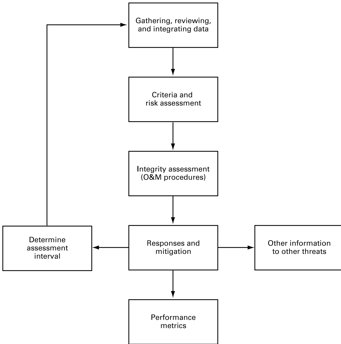
Figure A-8.1-1 Integrity Management Plan, Third-Party Damage Threat [Third-Party Inflicted Damage (Immediate), Vandalism, Previously Damaged Pipe; Simplified Process: Prescriptive]
