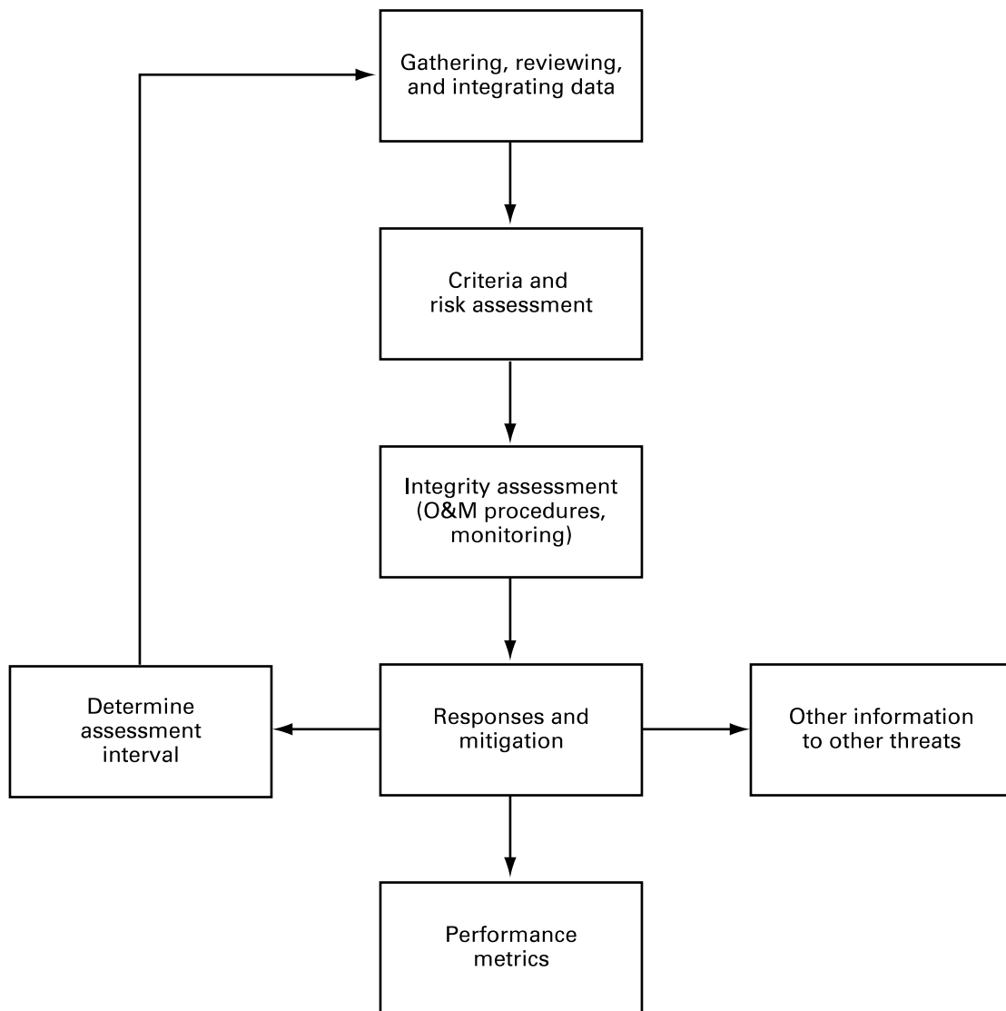
Figure A-10.1-1 Integrity Management Plan, Weather-Related and Outside-Force Threat (Earth Movement, Heavy Rains or Floods, Cold Weather, Lightning; Simplified Process: Prescriptive)
